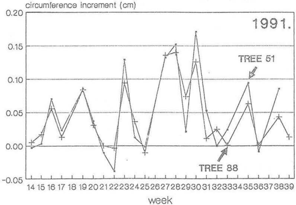
Fig. 3. Weekly circumference increment of two sessile oak stems
