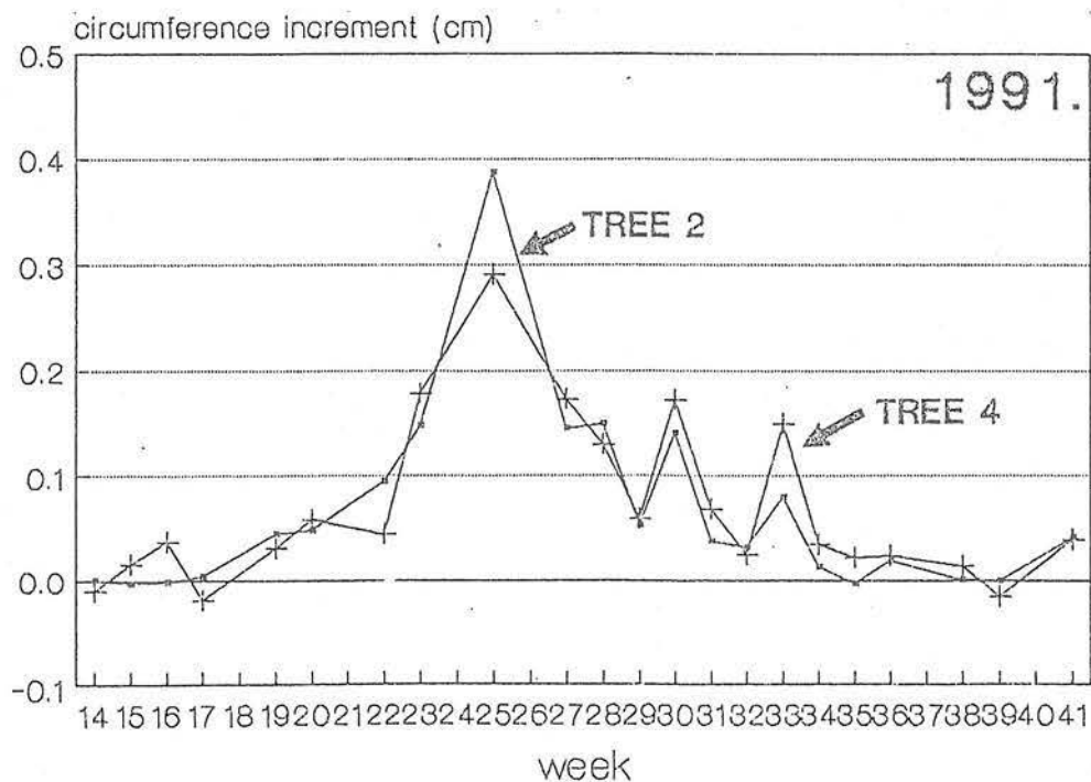
Fig.1. Weekly circumference increment of two beech stems
