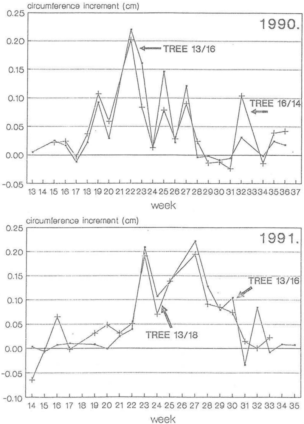
Fig.2. Weekly circumference increment of two spruce stems
